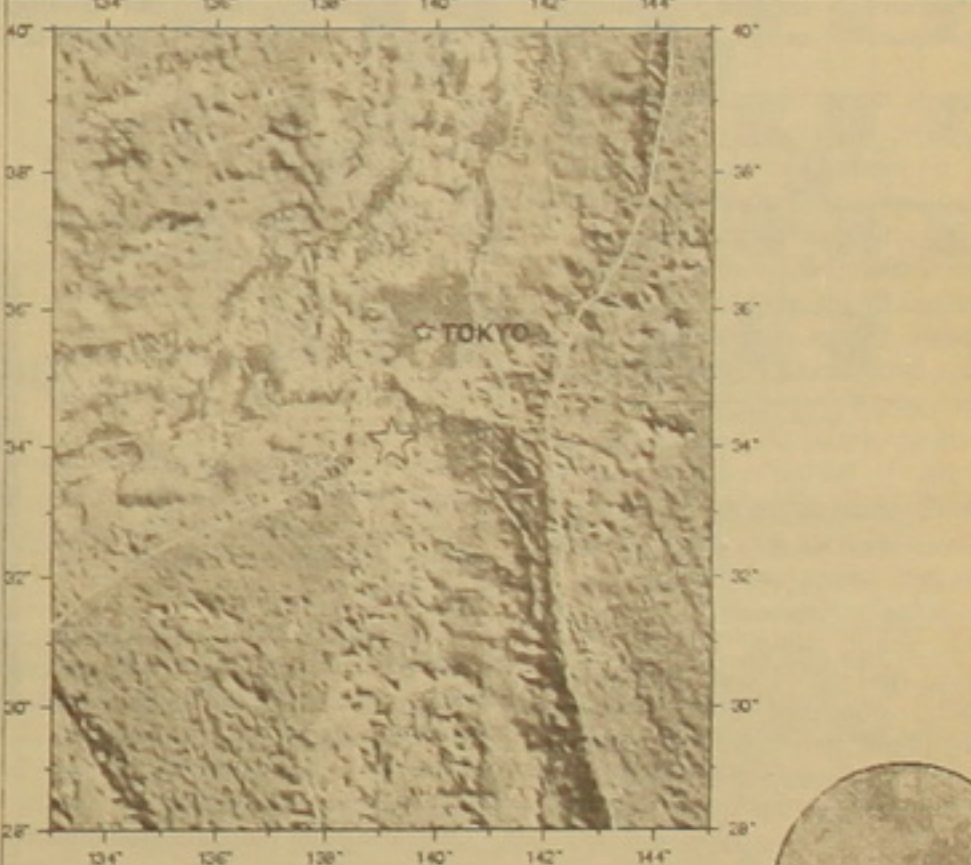
NEAR S. COAST OF HONSHU, JAPAN 00/07/13 18:55:55 UTC 34.05N 139.18E Depth: 33.0 km 5.0Mb USGS National Earthquake Information Center
